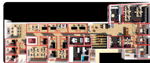
Office 105-2 is outlined on the plan.
